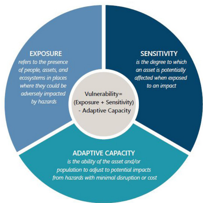
Vulnerability Equation
